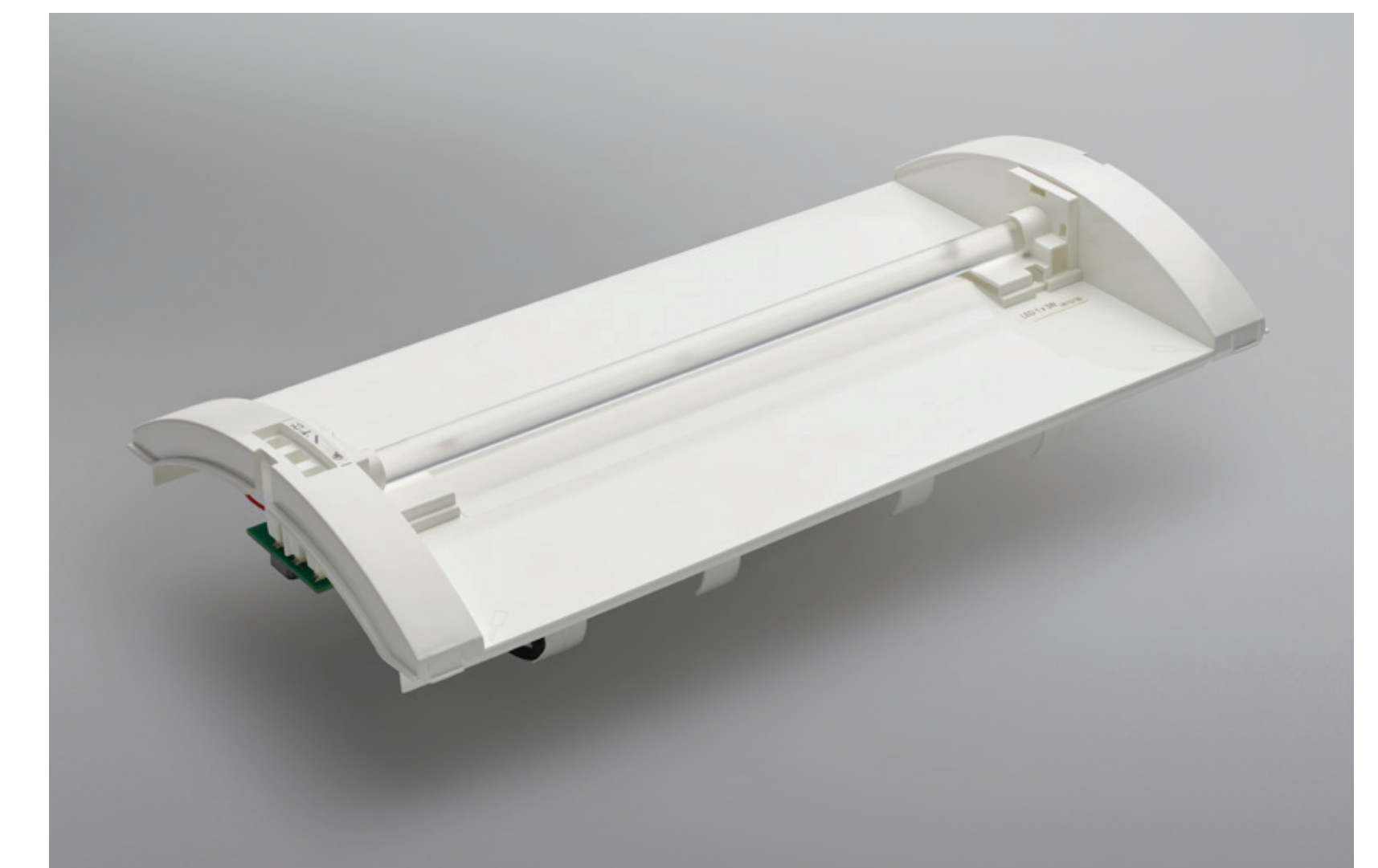
Renovation module with light guide (K1M32)
