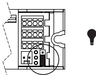
Non-maintained (daylight sensor not used)
